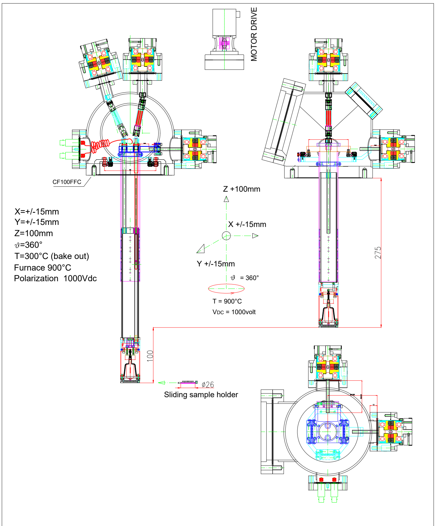
fig. 3 X-Y-Z Manipulator Mod XY15Z100TφV
